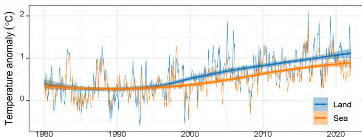
Figure 9 1: Trend in both land and sea temperature rise in Tanzania.
