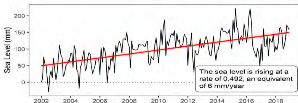
Figure 9-5: Sea level rise trend in rise in Dar es Salaam coastline since 2002.
