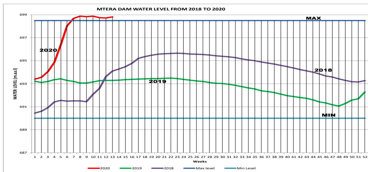
Figure 9-6: Trends in water levels at Mtera Dam from 2018 to 2020.
